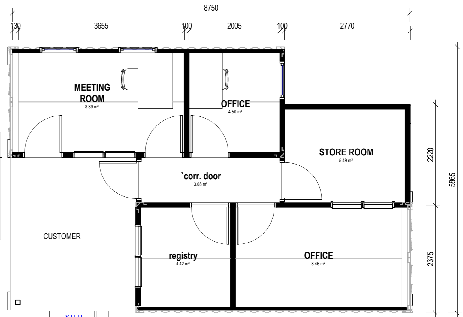
1 PROPOSED OFFICE PLAN CSNC LAYOUT 2815
