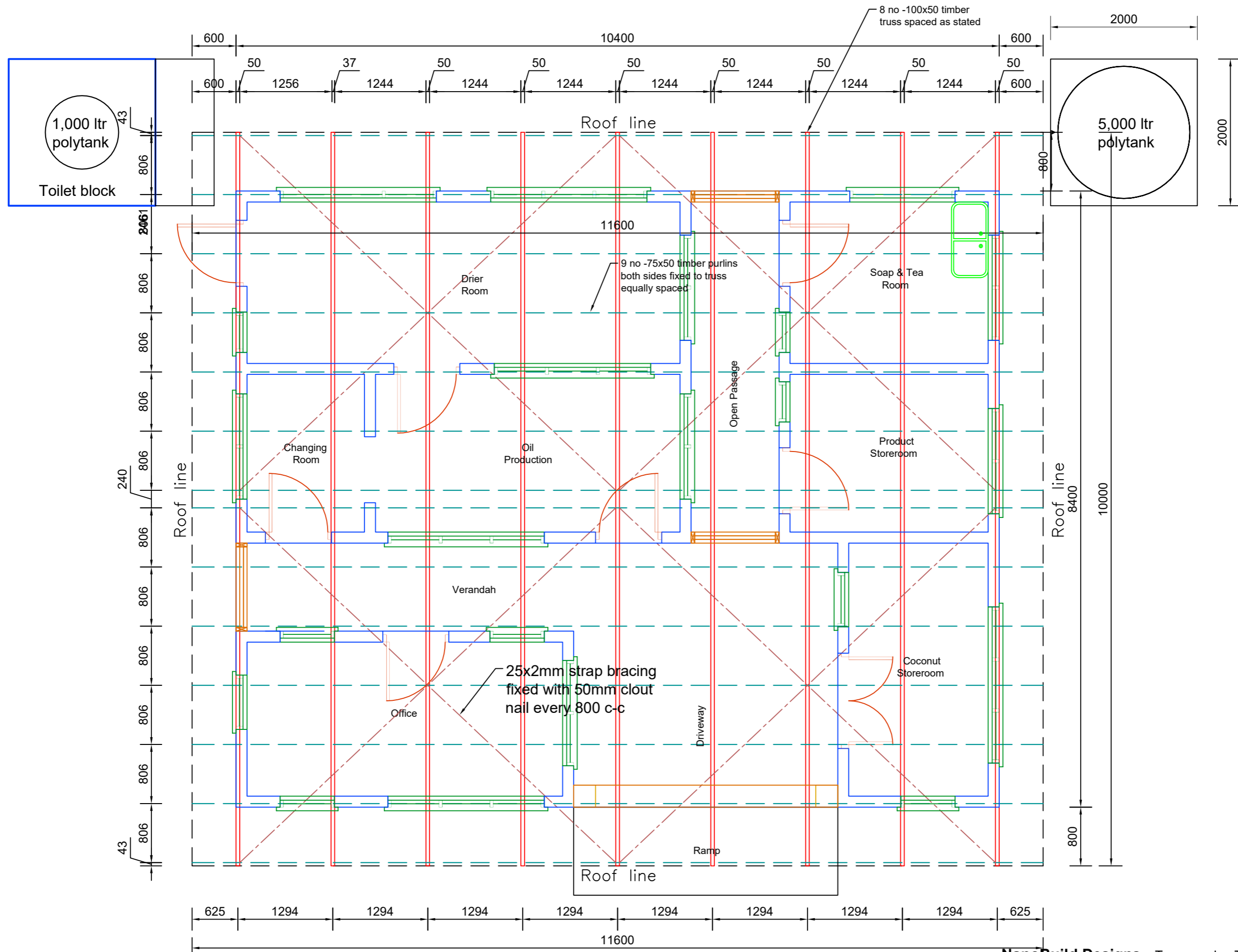
ROOFING PLAN Scale 1:50
