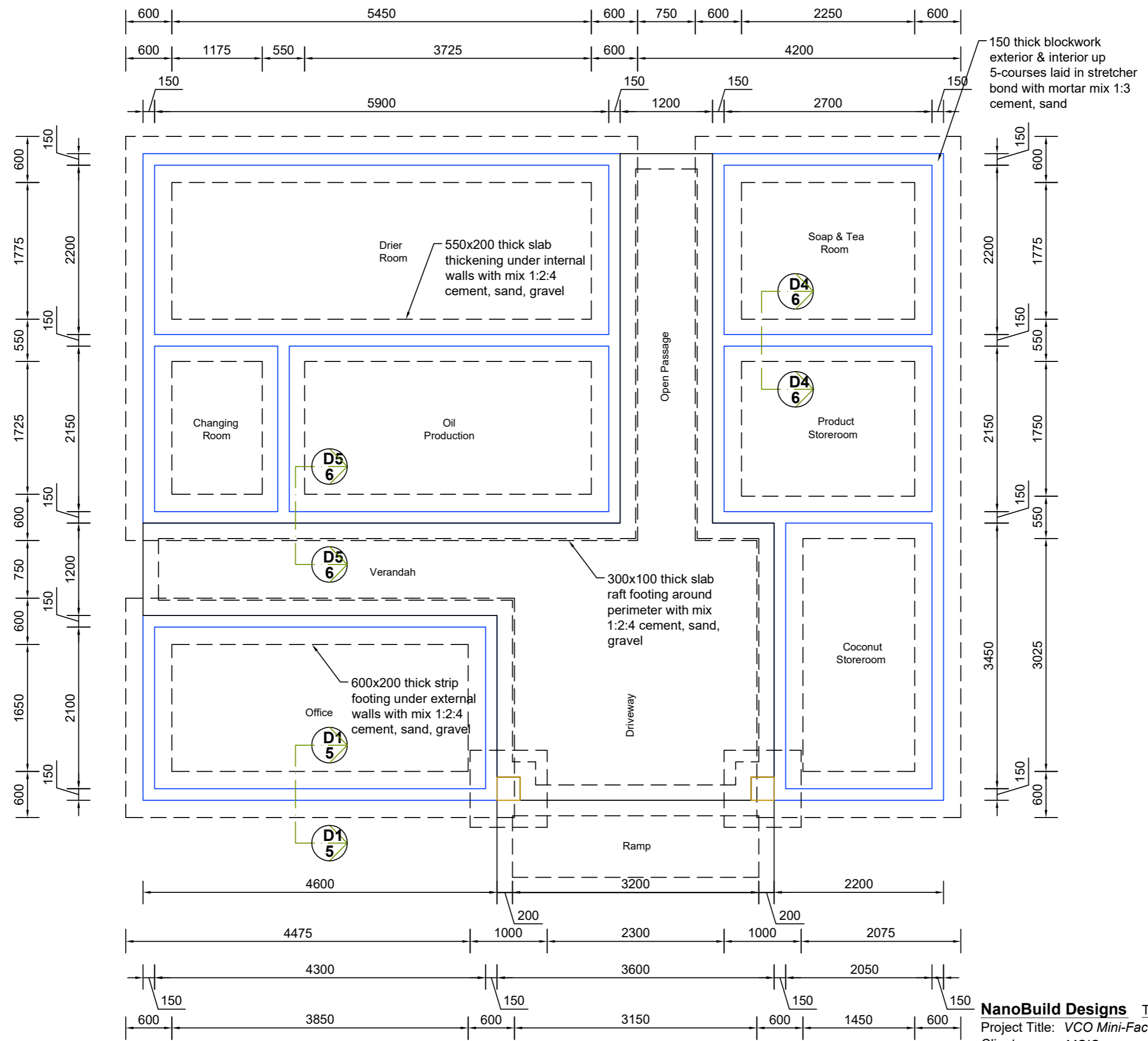
FOUNDATION PLAN Scale - NTS
